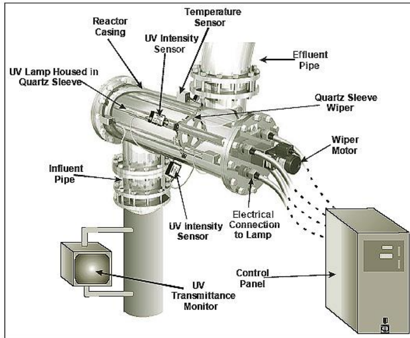
Figure 3. Continuous Flow UV Reactor Schematic (Source: Reference 2)
