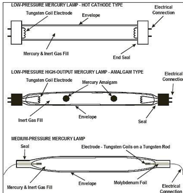
Figure 2. LP, LPHO, and MP Lamp Drawings (Source: Reference 2)
